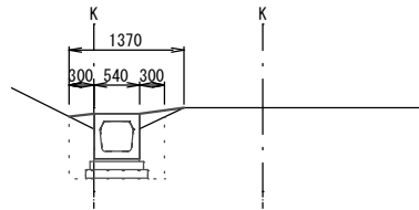
No.0+19.0(No.1)(同所) FH=1.31 GH=1.12
