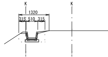
No.3+16.8(同所) FH=1.39 GH=1.32
