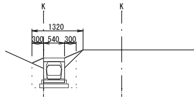
No.0+6.0 FH=1.25 GH=1.15
