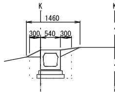
No.1+2.0 FH=1.31 GH=1.31
