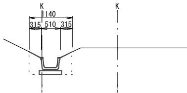
No.0+19.0(No.1) FH=1.12 GH=1.13
