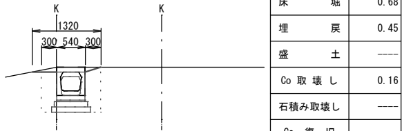
No.6+7.4 (同所) FH=1.82 GH=1.90
